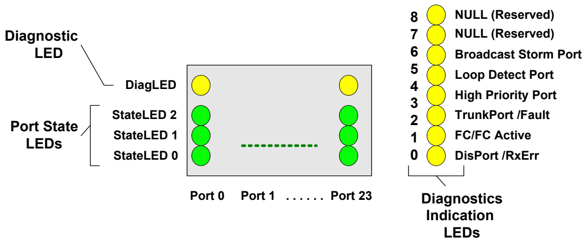
Figure 12. Serial LED Display
