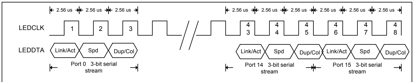
3-Bit Serial Stream Mode
